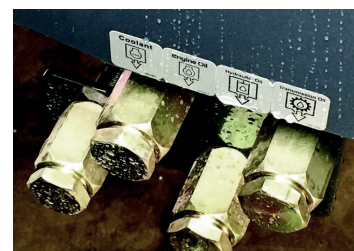
Autolube is a standard feature on the Taylor T-1023. All pressure taps and site gauges are easily accessible. Fluid drains provide environmentally friendly drainage capability and are grouped together for convenient serviceability.
