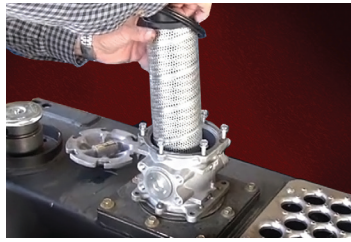
Spin-on Breather, Wire Mesh Strainer & Replaceable Internal Element (Standard)
